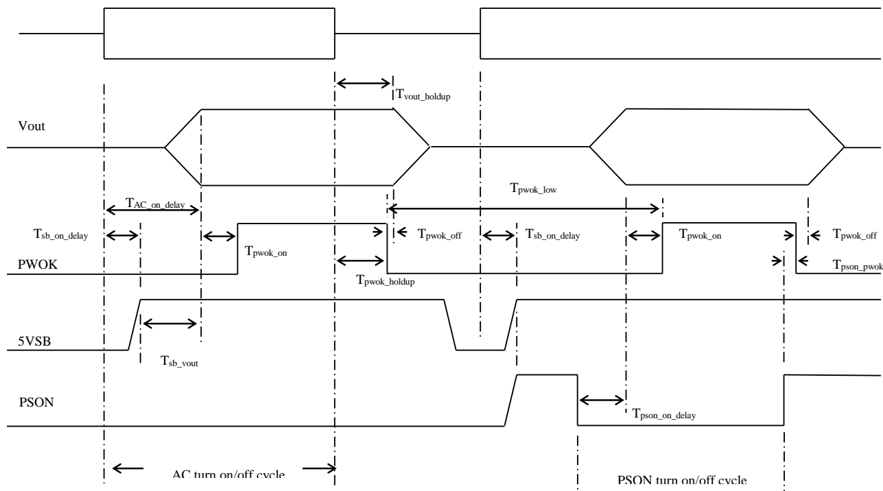
Figure 3 Timing Diagram
